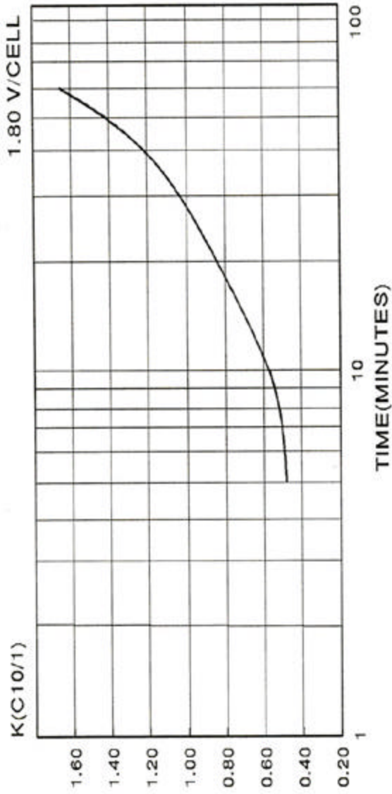
"K" CURVE ( 1.8 V/CELL)
